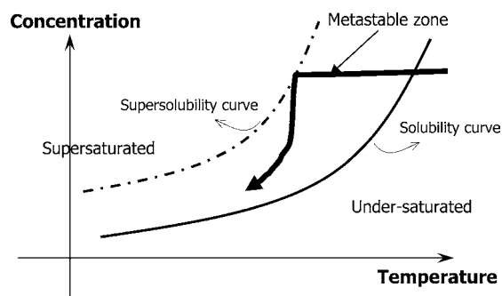
Figure 1. General schematic of a typical solution cooling crystallization process.
