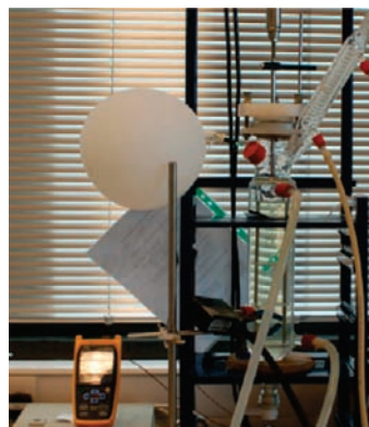
Figure 3. The setup of batch OBC.
